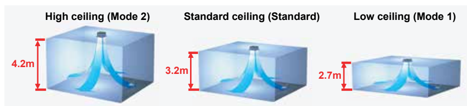
4-way Flow Adjustable modes
